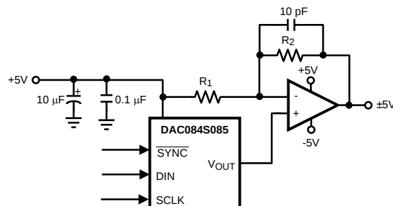
Figure 35. Bipolar Operation
