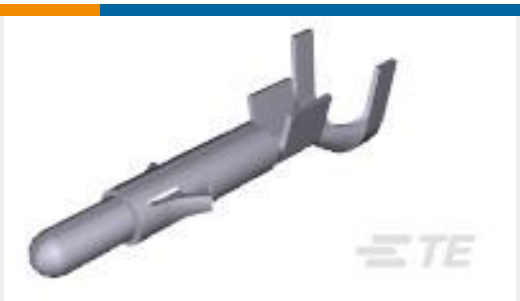
TE Part #350538-1 UMNL PIN 20-14 .0126 PTPBR
