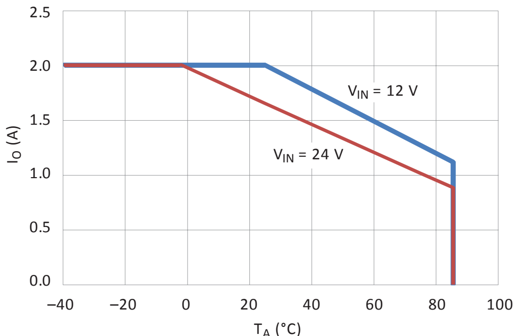
Figure 2. MPM80 thermal derating curve; measurement conditions: V_O = 5V , no heatsink
