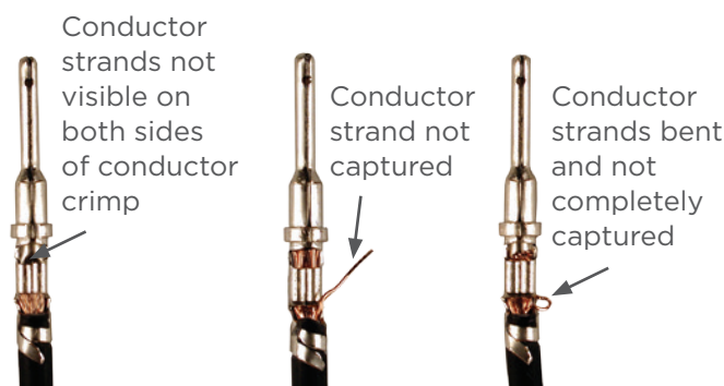
Unacceptable Crimps
