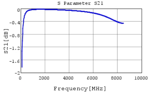
GRM0332C2A220JA01 S21 DCOV, 20degC
