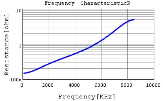
GRM0332C2A220JA01 R DCOV, 20degC
