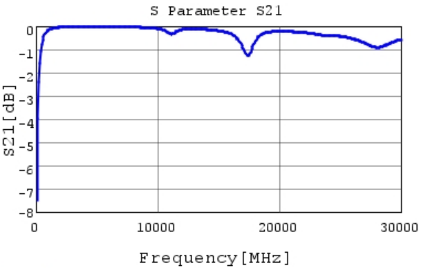
GJM0335C2A7R4WB01 S21 DCOV, 25degC
