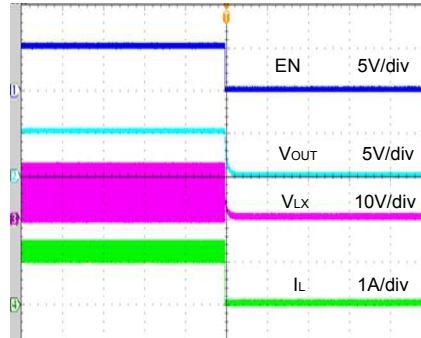
Shutdown From Enable ( V_{IN}=12V , V_{OUT}=5V , I_{LOAD}=1.2A )
