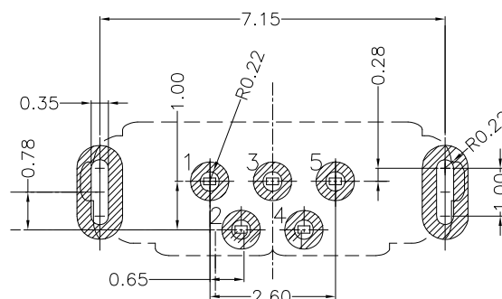
RECOMMEDED P.C.B LAYOUT
