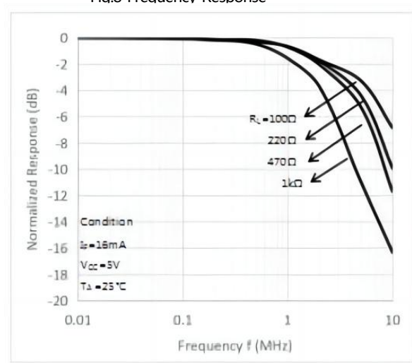
Fig.8 Frequency Response
