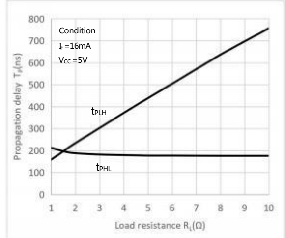
Fig.6 Propagation delay vs. Load resistance
