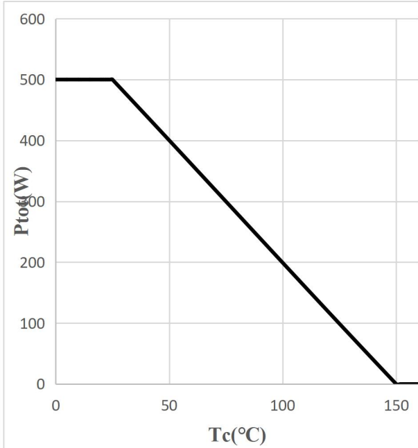
Figure 3: Power Dissipation
