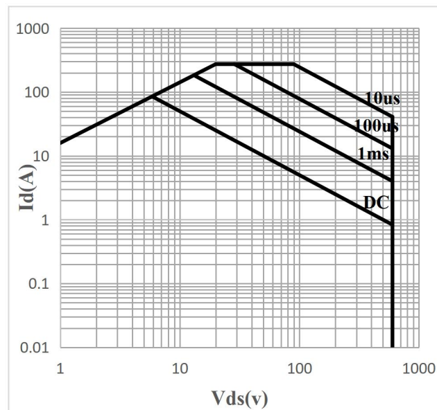
Figure 5: Safe Operating Area
