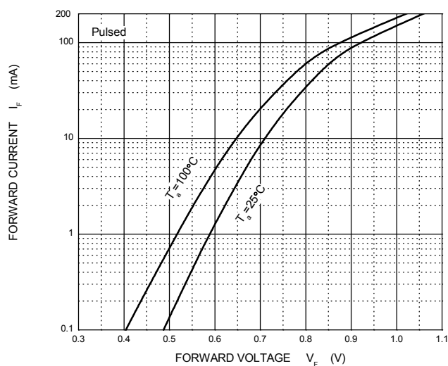
Forward Characteristics
