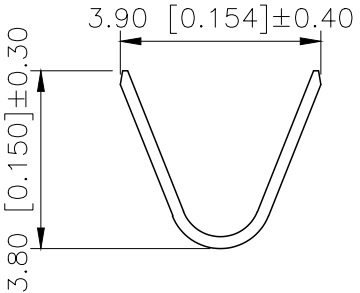
SECTION:A-A SCALE:1:1
