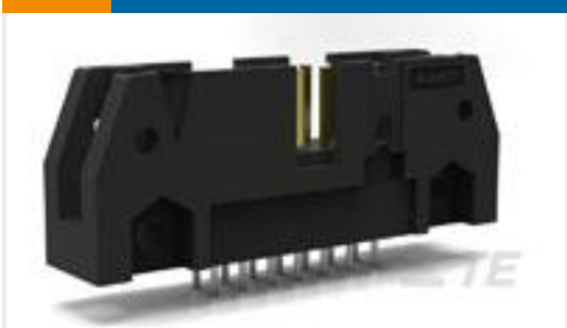
TE Part #5102153-4 A/L UNIV HDR 20P VERT
