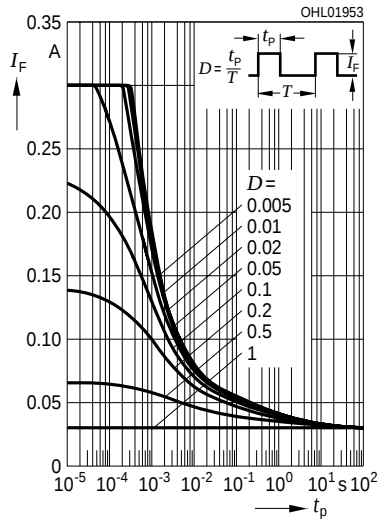
Zulässige Impulsbelastbarkeit I_F = f(t_p) Permissible Pulse Handling Capability Duty cycle D = parameter, T_A = 25^\circ\text{C} , LT / LV
