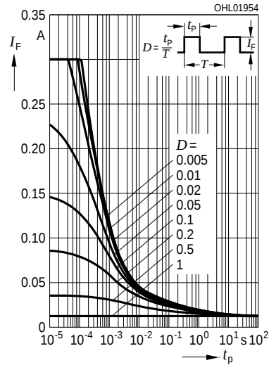
Zulässige Impulsbelastbarkeit I_F = f(t_p) Permissible Pulse Handling Capability Duty cycle D = parameter, T_A = 85^\circ\text{C} , LT / LV
