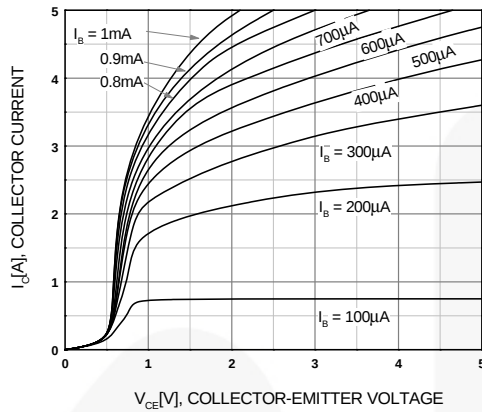
Figure 1. Static Characteristic
