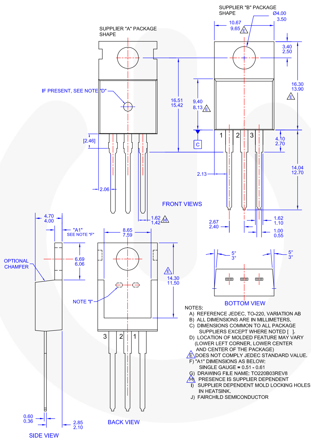
Figure 7. TO-220, MOLDED, 3LEAD, JEDEC VARIATION AB
