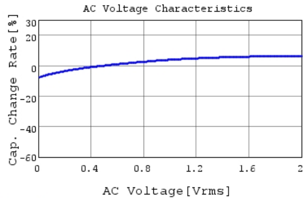
GRM155R61A334ME15 C-AC Voltage capchange, DC
