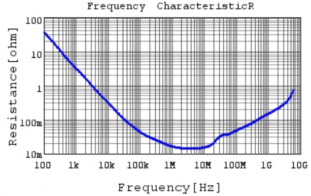
GRM155R61A334ME15 R DCOV, 25degC
