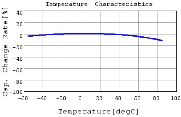
GRM155R61A334ME15 C-Temp. capchange, DC0.0V,
