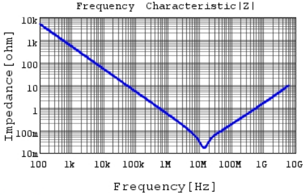
GRM155R61A334ME15 |Z| DCOV, 25degC
