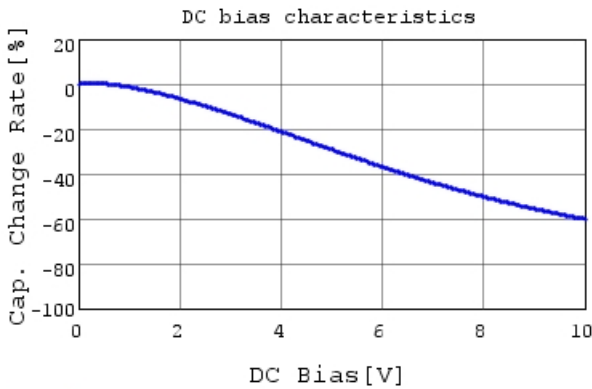
GRM155R61A334ME15 C-DC bias capchange, 25.0c
