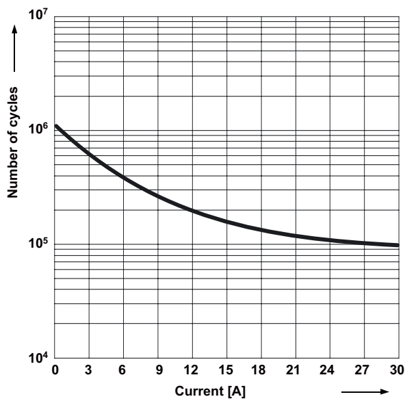
Electrical life at 250 VAC, resistive load
