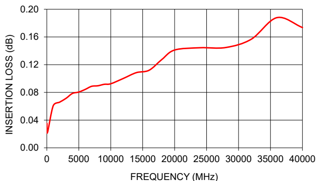
KFFL-KF50+ INSERTION LOSS
