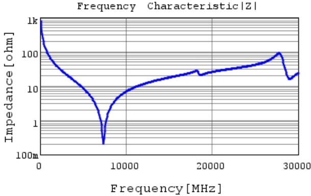
GJM0335C1H2R0WB01 |Z| DCOV, 25degC
