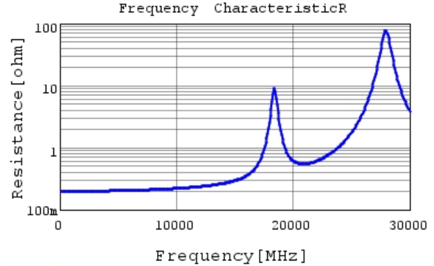
GJM0335C1H2R0WB01 R DCOV, 25degC
