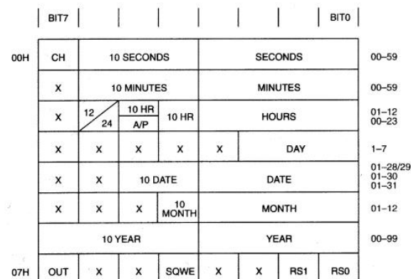
DS1307ZN TIMEKEEPER REGISTERS Figure 3
