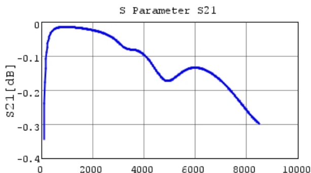
■ GRT0335C1H560FA02 S21 DCOV, 25degC
