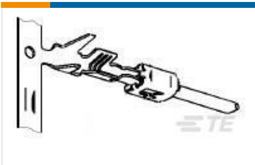
TE Part #2-2141598-2 TAB 2.8x0.8 CONTACT CF SRC Ag
