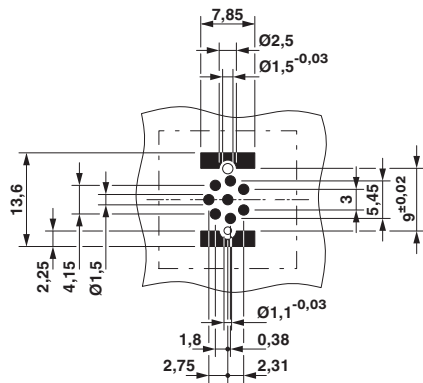
Drilling diagram
