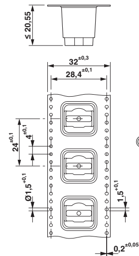
Dimensional drawing
