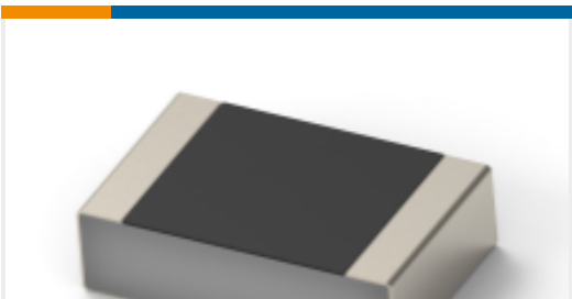
TE Part #2-2176452-3 CPF 0201 909R 0.1% 25ppm 1K RL
