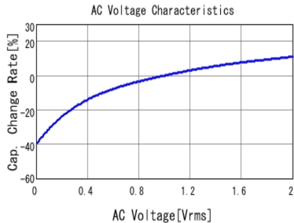
■ GRM155R71A224KE01 C-AC Voltage capchange, DC0V, 25.0d
