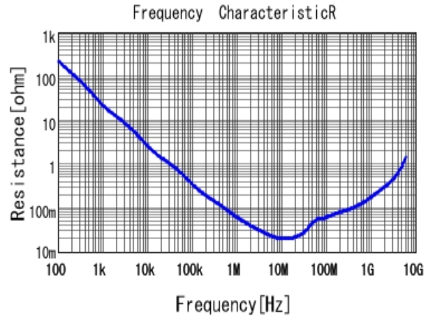
■ GRM155R71A224KE01 R DC0V, 25degC
