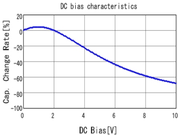
■ GRM155R71A224KE01 C-DC bias capchange, 25.0degC, AC1.
