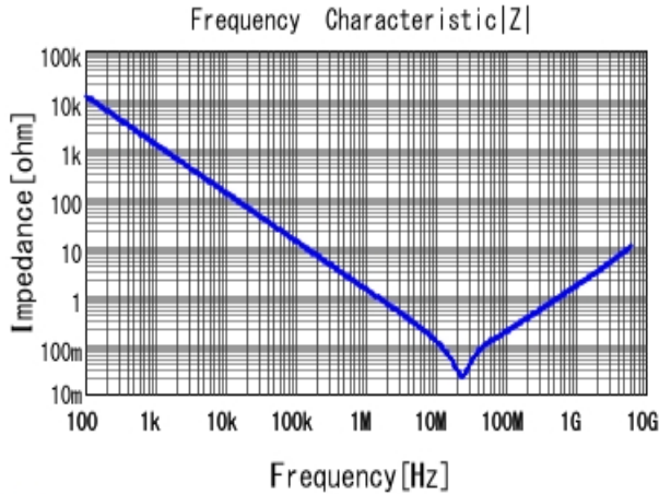
■ GRM155R71A224KE01 |Z| DC0V, 25degC
