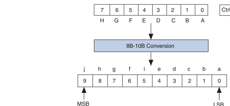
Figure 2-6. 8B/10B Encoder
