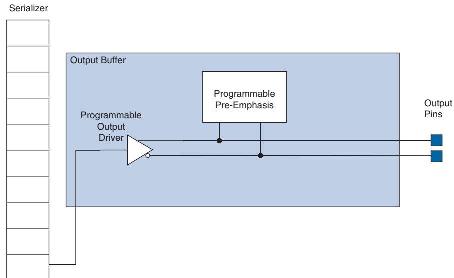
Figure 2-8. Output Buffer
