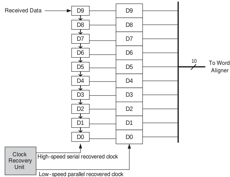
Figure 2-14. Deserializer (Note 1)
