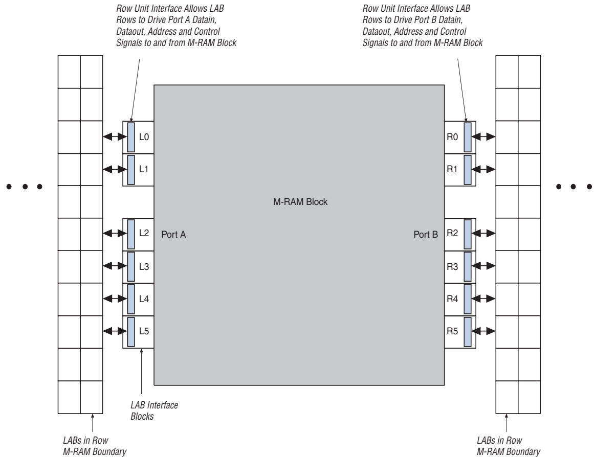
Figure 2-48. M-RAM Block LAB Row Interface (Note 1)
