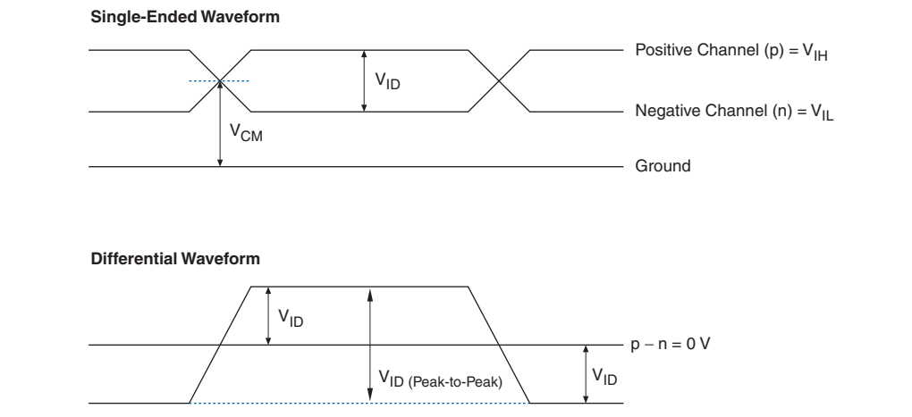
Figure 4-5. Receiver Input Waveforms for Differential I/O Standards
