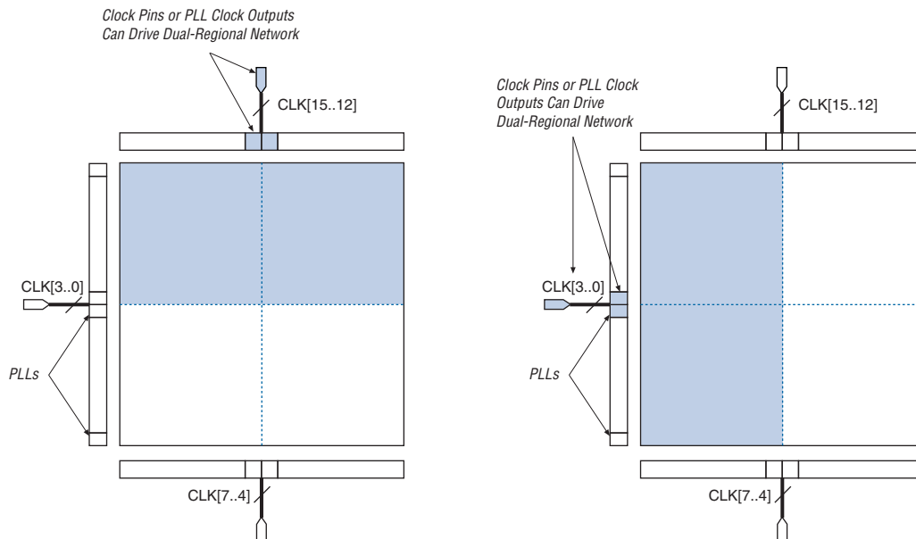
Figure 2-56. Dual-Regional Clocks
