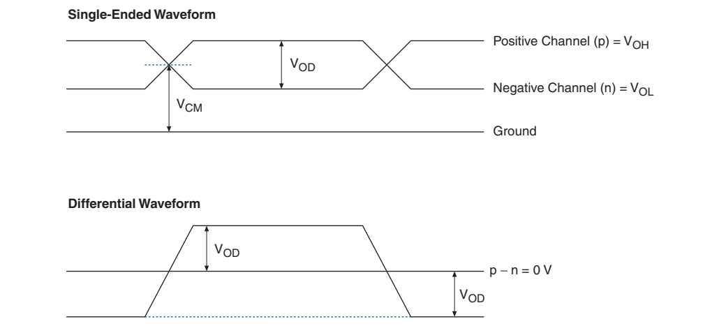
Figure 4-6. Transmitter Output Waveforms for Differential I/O Standards
