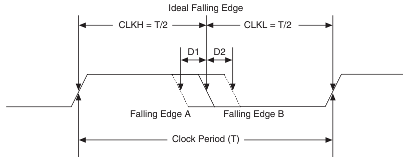
Figure 4-10. Duty Cycle Distortion
