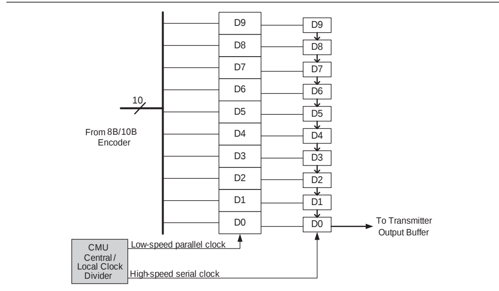
Figure 2-7. Serializer
