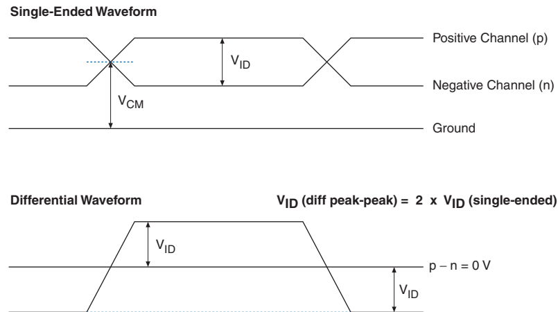
Figure 4-3. Receiver Input Waveform
