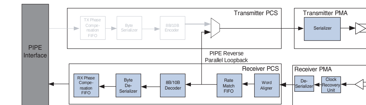
Figure 2-21. PCI Express (PIPE) Reverse Parallel Loopback
