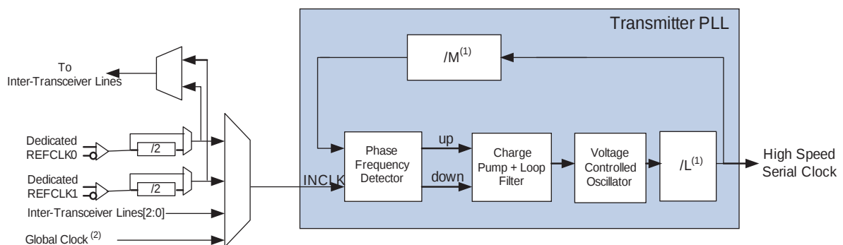
Figure 2-4. Transmitter PLL
