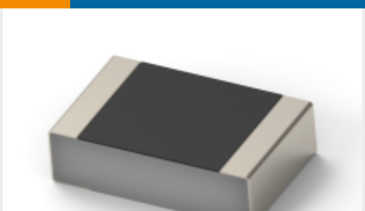
TE Part #7-2176453-5 CPF 0201 34K 0.1% 25ppm 1K RL
