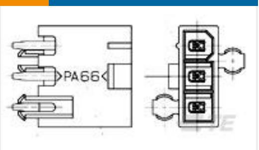
TE Part #2029181-3 3P VAL-U-LOK VRTHDR W/PGS GW
