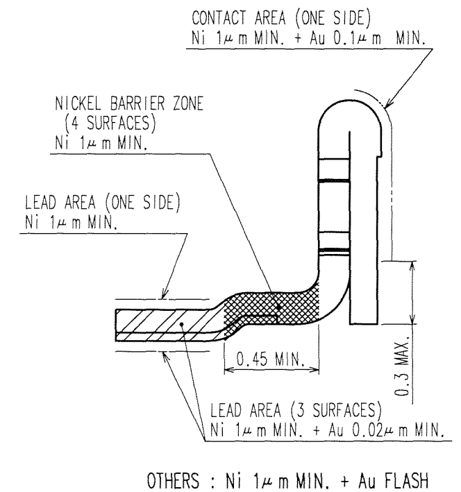
Fig.2 : PLATING SPECIFICATION (40:1)
