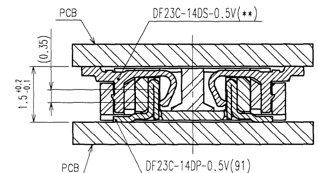
Fig.4 : MATING VIEW
