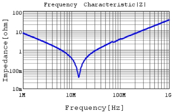
RCE5C2E223J2M1H03A |Z| DCOV, 25degC
