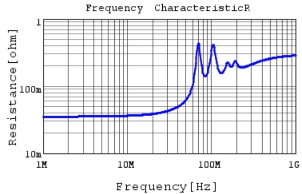
RCE5C2E223J2M1H03A R DCOV, 25degC
