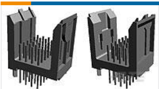
TE Part #1776302-1 TSB100001DS=EUROPA TM BLK, 12MM
