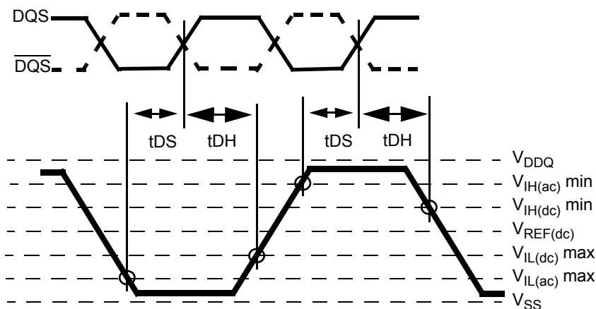
< Differential Input waveform timing >
