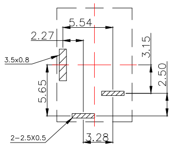
PCB.WELDING DRAWING (TOLERANCE: ±0.05)
