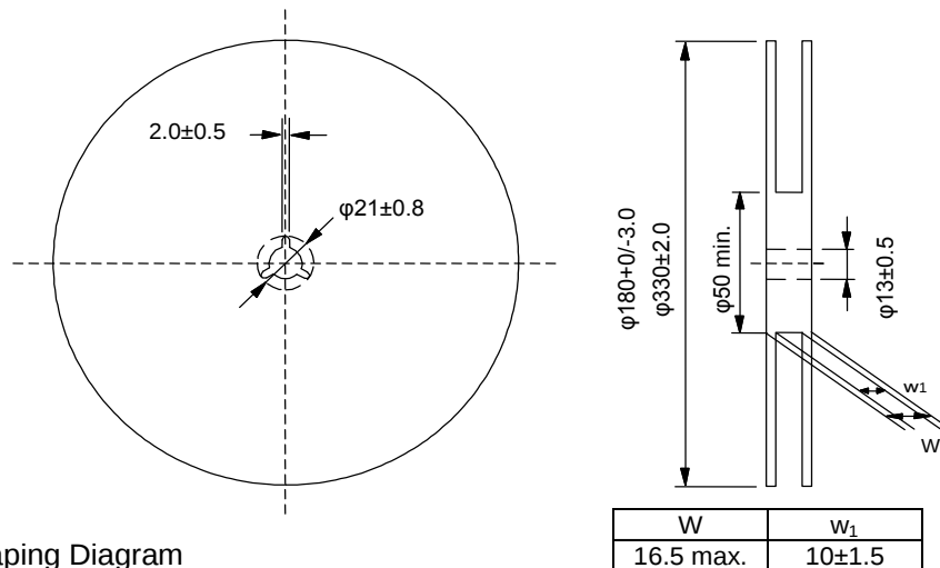
Fig.2 Dimensions of Reel
