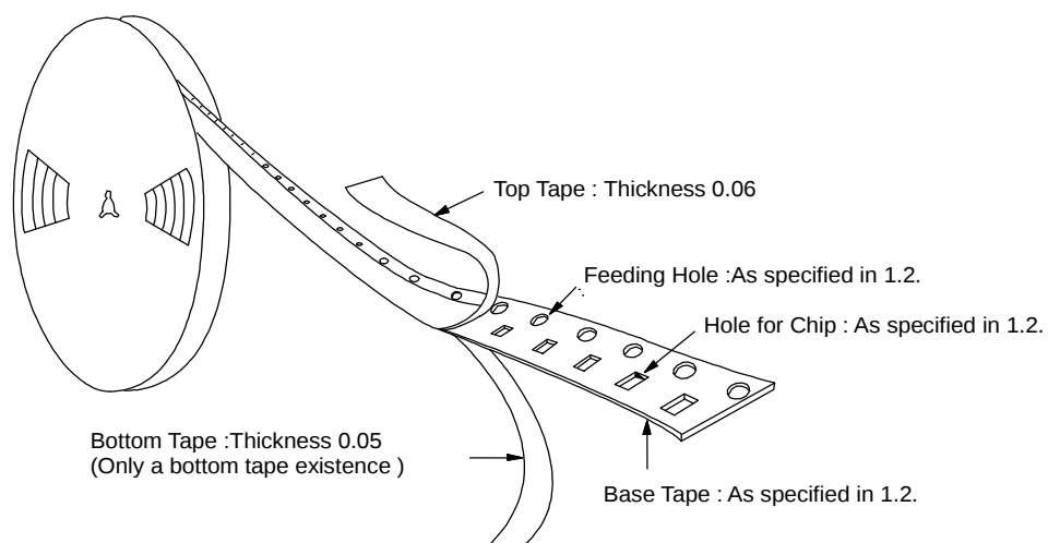
Fig.3 Taping Diagram
