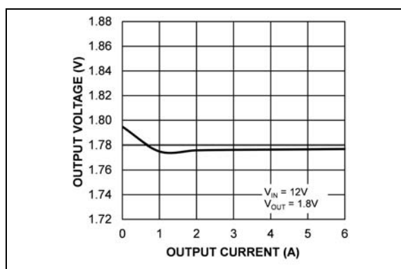
FIGURE 2-26: Output Voltage vs. Output Current (MIC45116-1).
