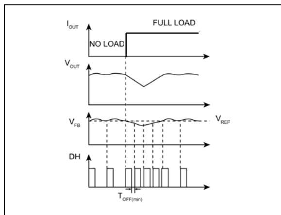
FIGURE 4-3: MIC45116 Load Transient Response.
