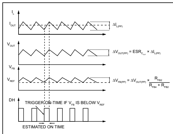
FIGURE 4-2: MIC45116 Control Loop Timing.
