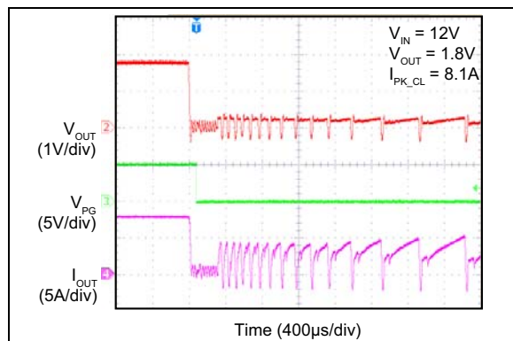
FIGURE 2-49: Peak Current-Limit Threshold.
