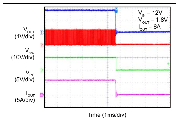
FIGURE 2-51: Thermal Shutdown.
