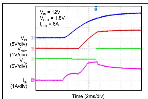
FIGURE 2-50: Inrush with 3000 \mu F.
