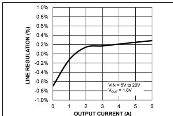
FIGURE 2-25: Line Regulation vs. Output Current (MIC45116-1).
