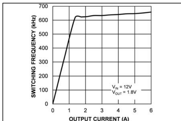
FIGURE 2-27: Switching Frequency vs. Output Current (MIC45116-1).
