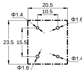
Reference Hole Pattern
