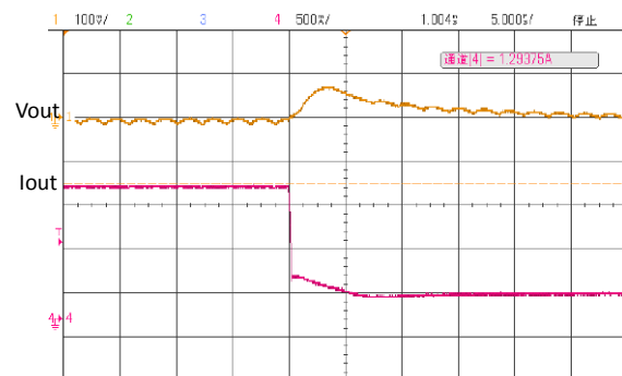
Load Transient Response – Iout Falling Edge 1A/0.2us Vin=12V, Vout=1.1V, L=2.2uH, Cout=22uF, Iout 1.5-0.3A
