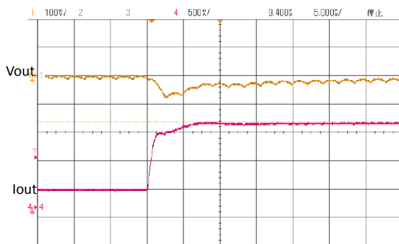
Load Transient Response – Iout Rising Edge 1A/1us Vin=12V, Vout=1.1V, L=2.2uH, Cout=22uF, Iout 0.3-1.5A
