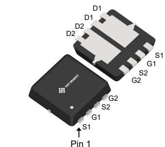
DFN3X3B-8L
