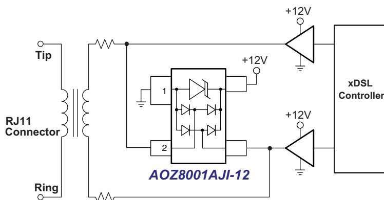
Figure 2. xDSL Application
