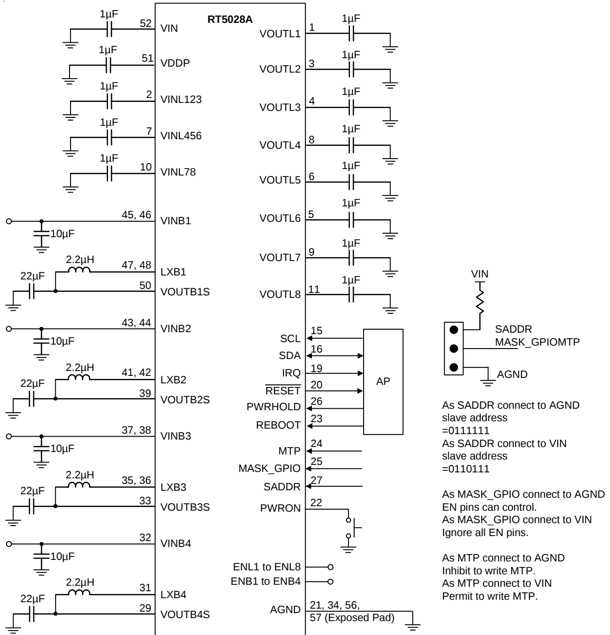
Suggested Components for Typical Application Circuit
