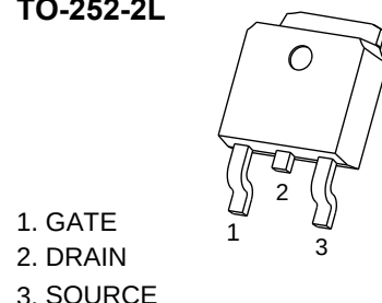
TO-252-2L
