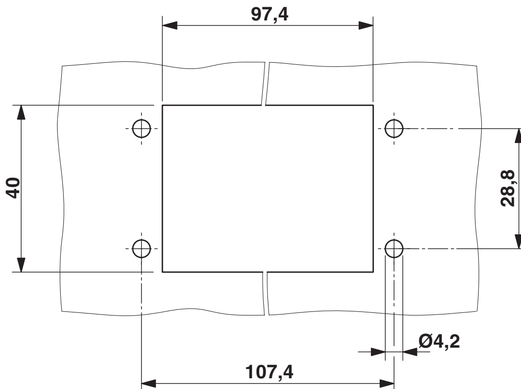
Dimensional drawing
