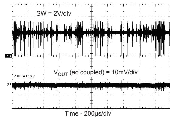
Figure 22. Pulse Skipping
