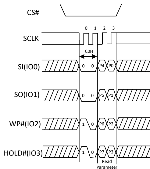
Figure 32. Set Read Parameters command Sequence Diagram
