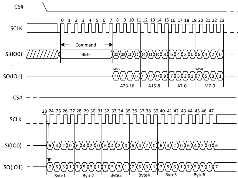
Figure 10. Dual I/O Fast Read Sequence Diagram
