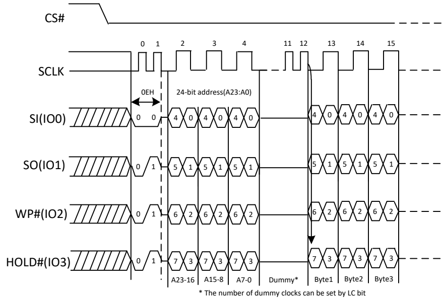
Figure 15. DTR Burst Read With Wrap command Sequence Diagram (QPI)
