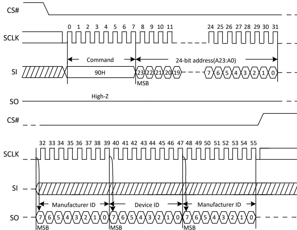
Figure 3. Read Manufacture ID/ Device ID Sequence Diagram
