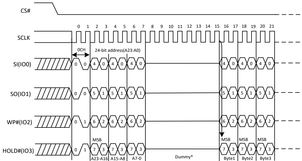
Figure 13. Burst Read with Wrap command Sequence Diagram (QPI)
