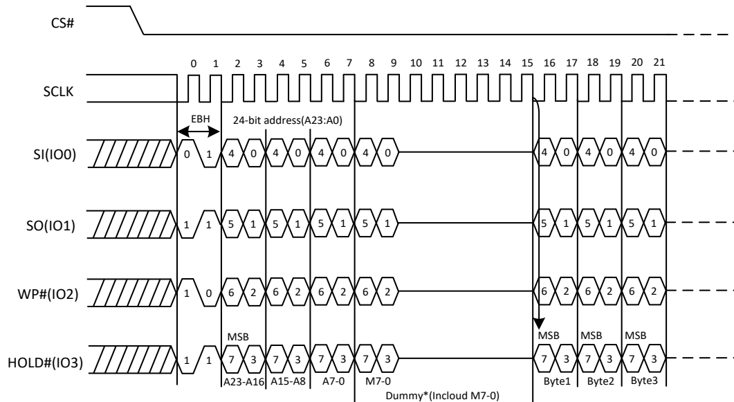
Figure 12b. Quad I/O Fast Read Sequence Diagram (QPI)
