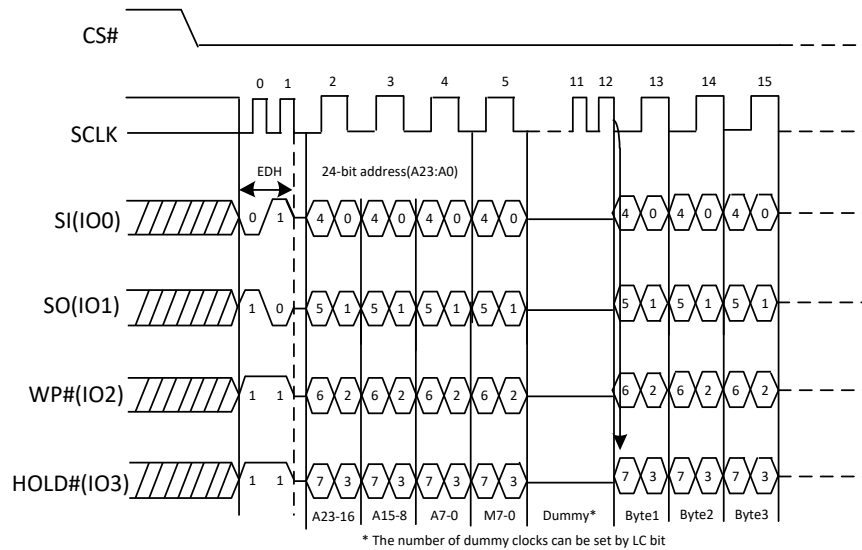
Figure 14a. DTR Fast Read Quad I/O (QPI)
