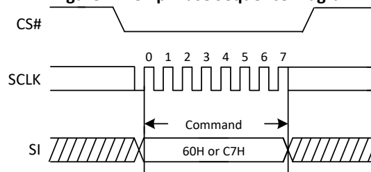
Figure 22. Chip Erase Sequence Diagram
