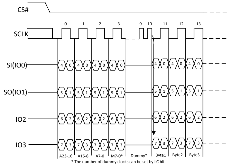
Figure 14. DTR Fast Read Quad I/O
