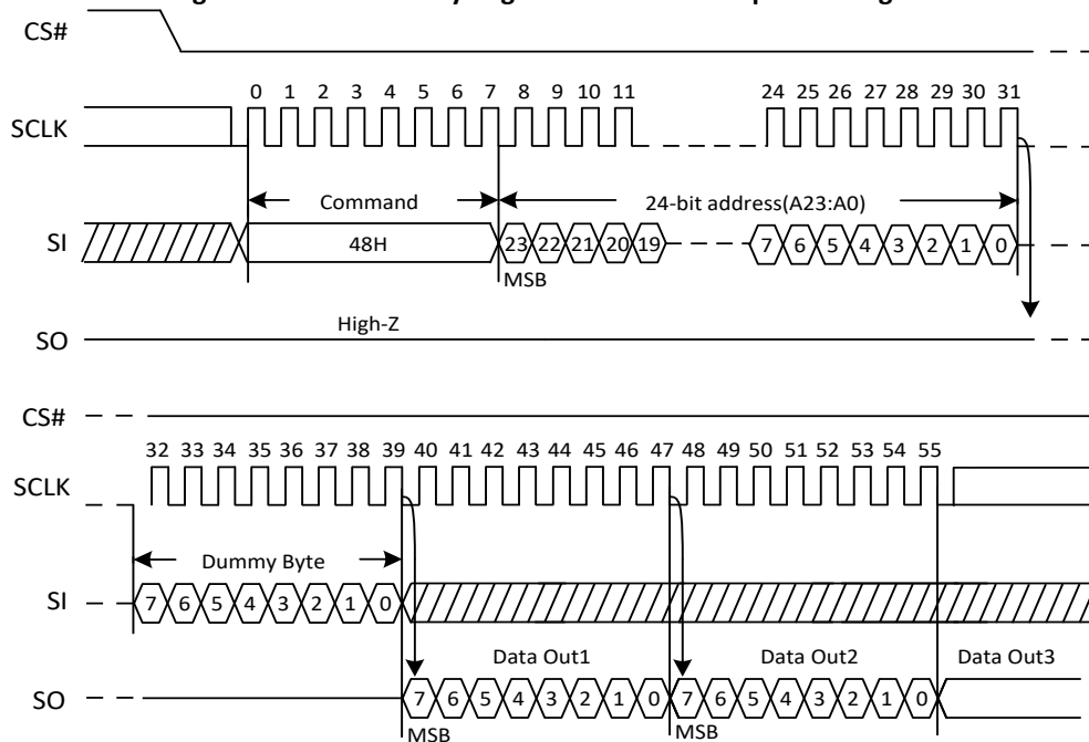
Figure 35. Read Security Registers command Sequence Diagram
