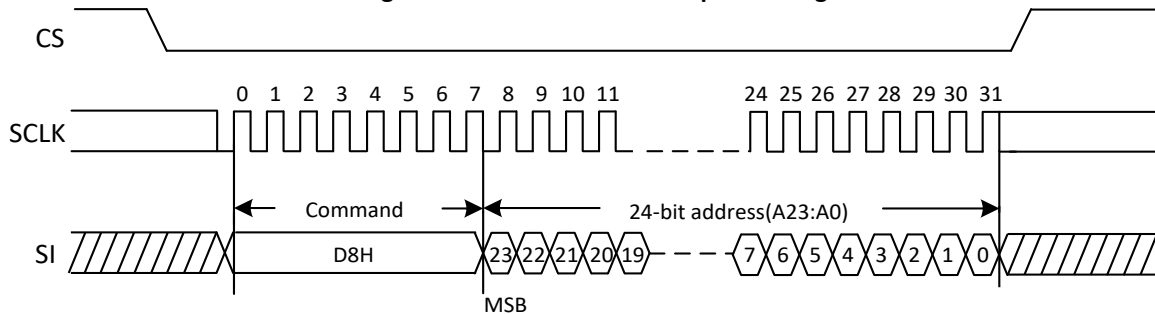
Figure 21. 64KB Block Erase Sequence Diagram
