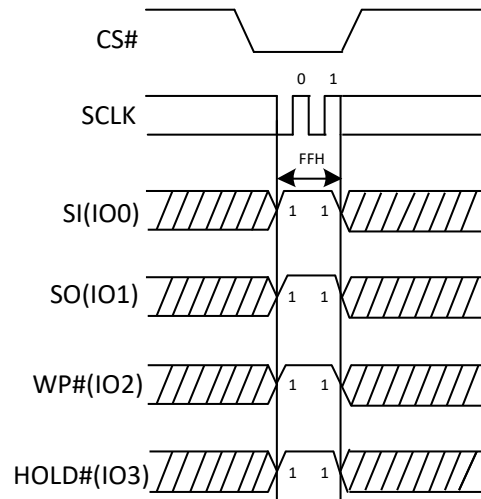
Figure 30. Disable QPI mode command Sequence Diagram
