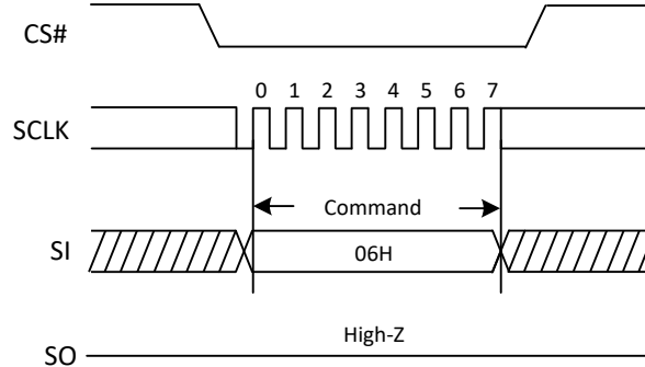
Figure 24. Write Enable Sequence Diagram
