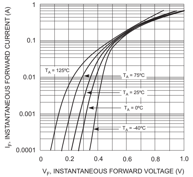
Fig. 2 Forward Characteristics
