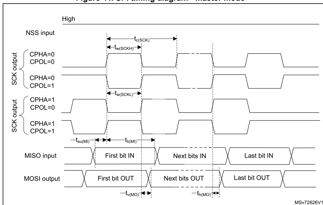
Figure 44. SPI timing diagram - master mode (1)
