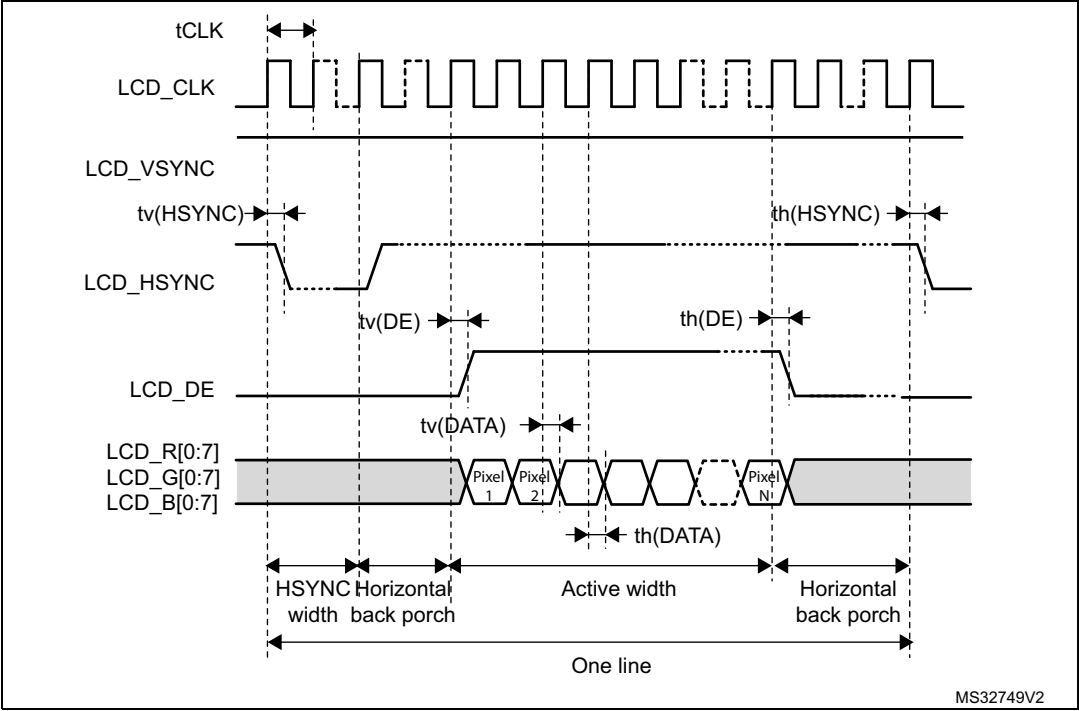
Figure 40. LCD-TFT horizontal timing diagram
