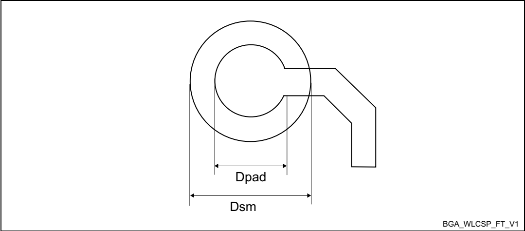
Figure 63. TFBGA289 - Recommended footprint
