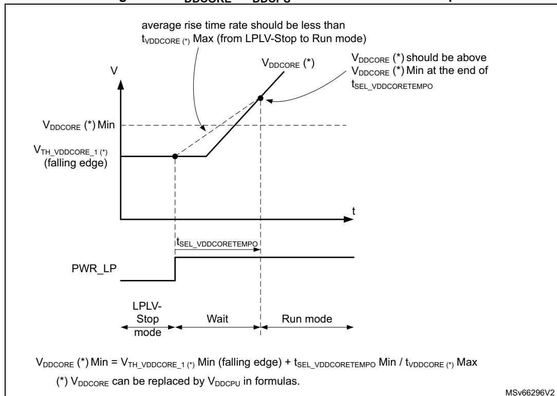
Figure 13. V_{DDCORE} / V_{DDCPU} rise time from LPLV-Stop
