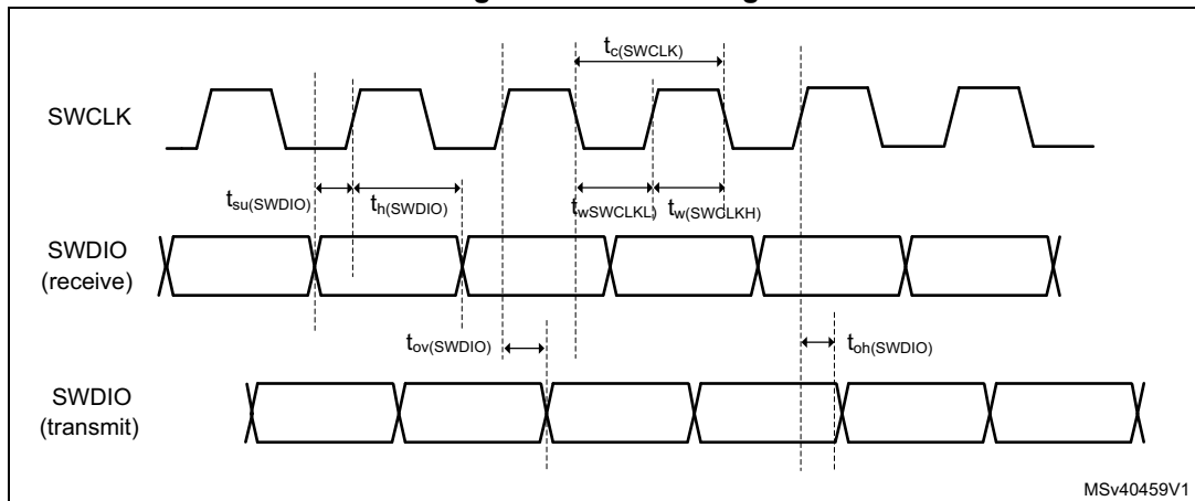
Figure 59. SWD timing
