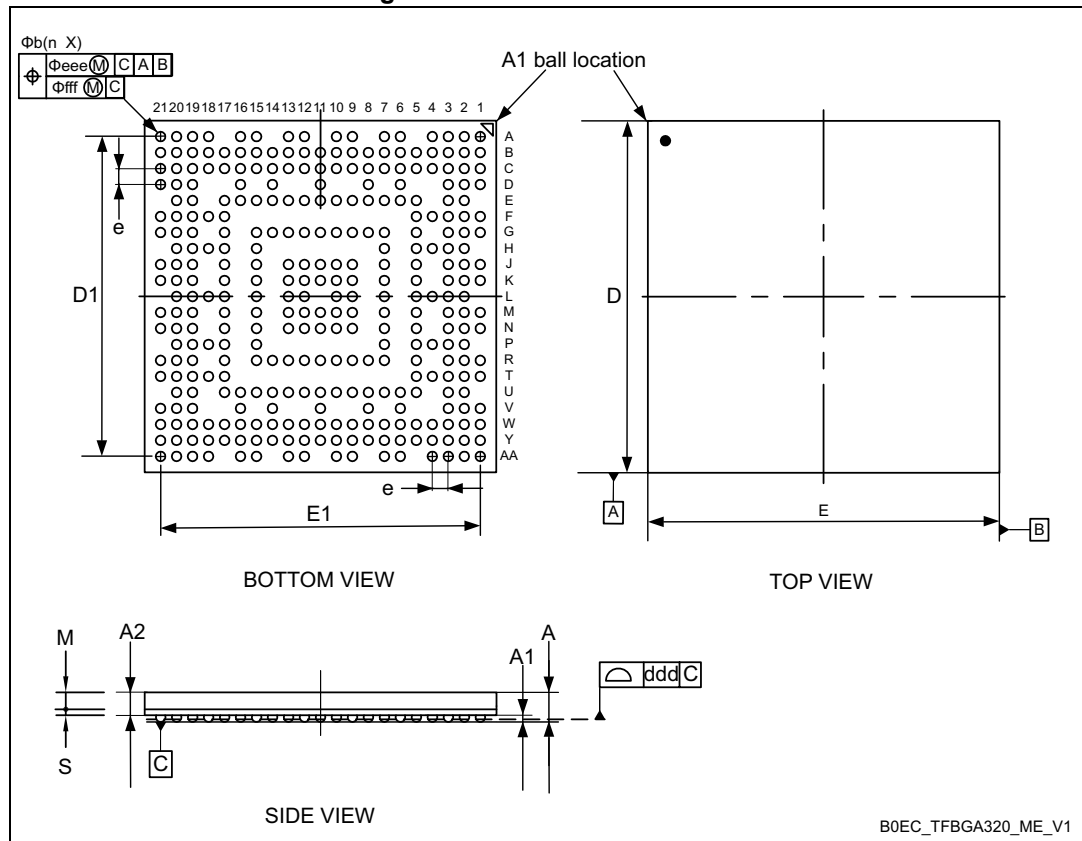
Figure 64. TFBGA320 - Outline
