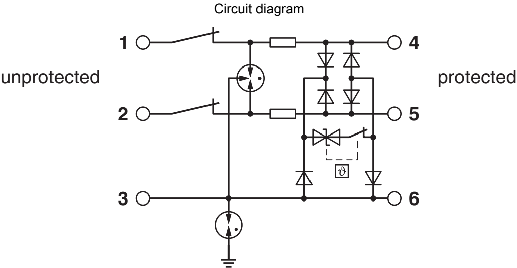
Schematic diagram
