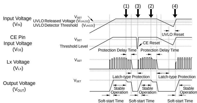
Timing Chart
