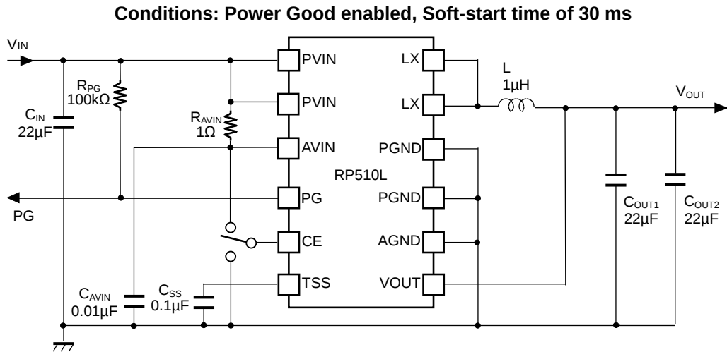
RP510Lxx1G/1H/4G/4H (Fixed Output Voltage Type) Typical Application Circuit
