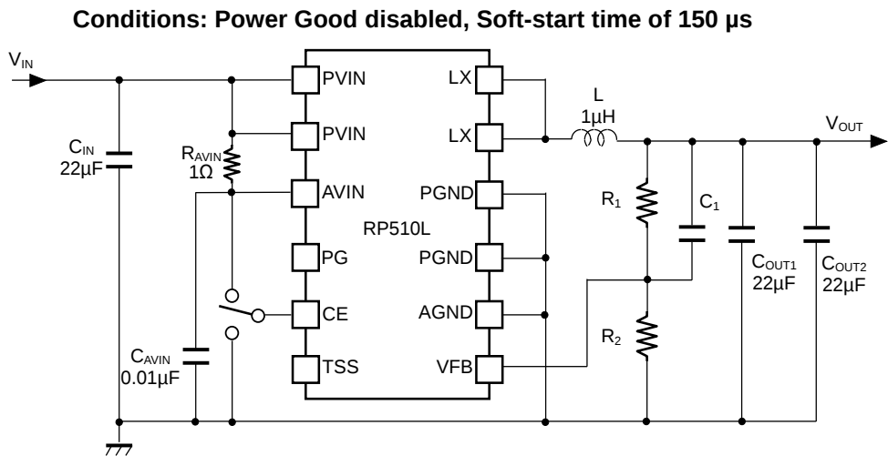
RP510L001J/1N/4J/4N (Adjustable Output Voltage Type) Typical Application Circuit
