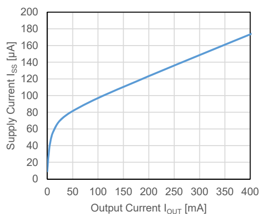
RP122x281x, V_{IN} = 3.8 V
