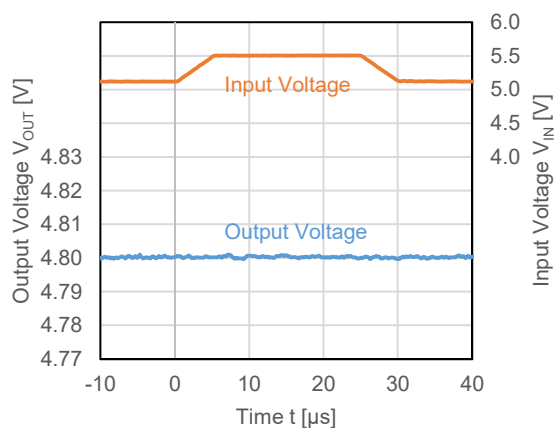
RP122x481x, I_{OUT} = 1 \text{ mA}
