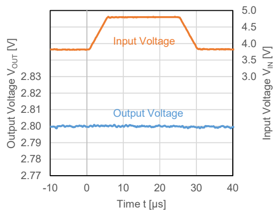
RP122x481x, I_{OUT} = 20 \text{ mA}
