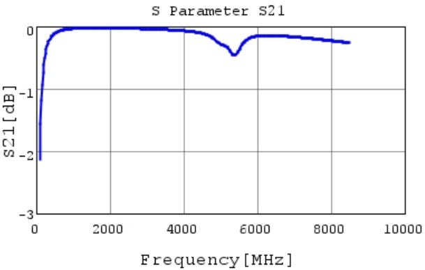
GCM0335C1E200FA16 S21 DCOV, 25degC
