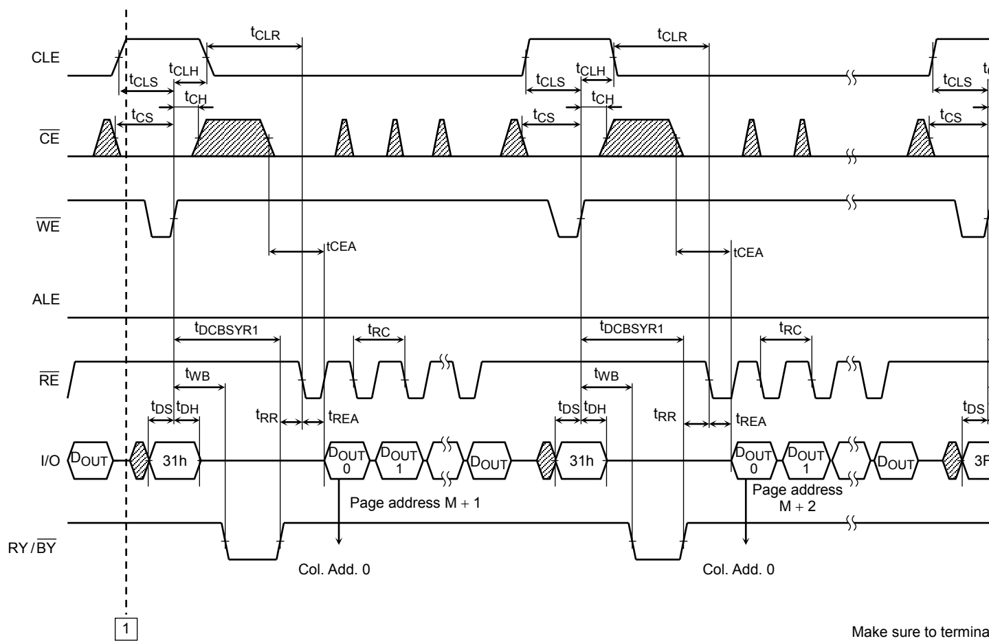
Read Cycle with Data Cache Timing Diagram (2/2)
